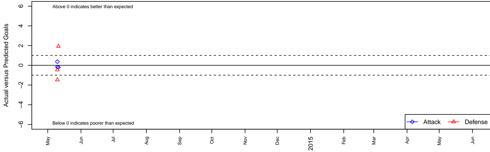
XUnk U12g Red G01 Dots are actual minus expected GF (blue circles) and GA (red triangles). Blue line is smoothed change in attack strength. Red is smoothed change in defense strength.
